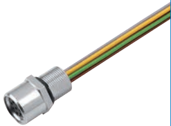
Female panel mount connector with single wires, 8 x 0,14 mm 2
